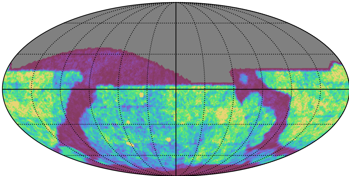
weather_cloudso8v3.4_10yrs i band: Gaps_24hr
