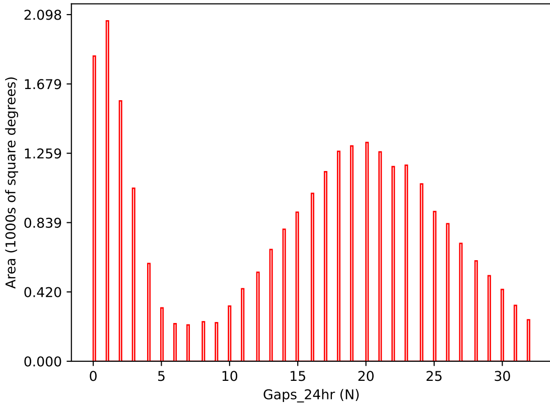
weather_cloudso8v3.4_10yrs i band: Gaps_24hr
