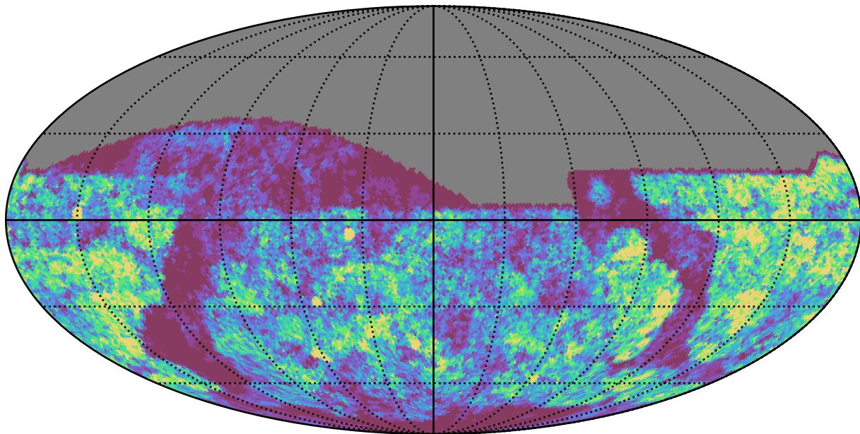
weather_cloudso8v3.4_10yrs g band: Gaps_24hr
