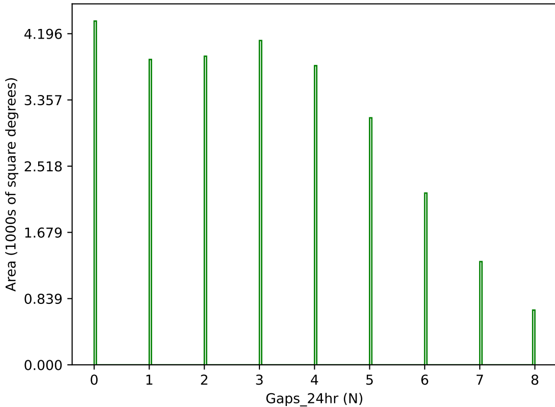
weather_cloudso8v3.4_10yrs g band: Gaps_24hr
