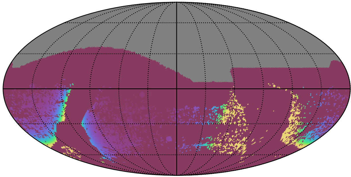
weather_cloudso8v3.4_10yrs : GalplaneFootprintMetric_xray_binaries_map_Tau_5_0
