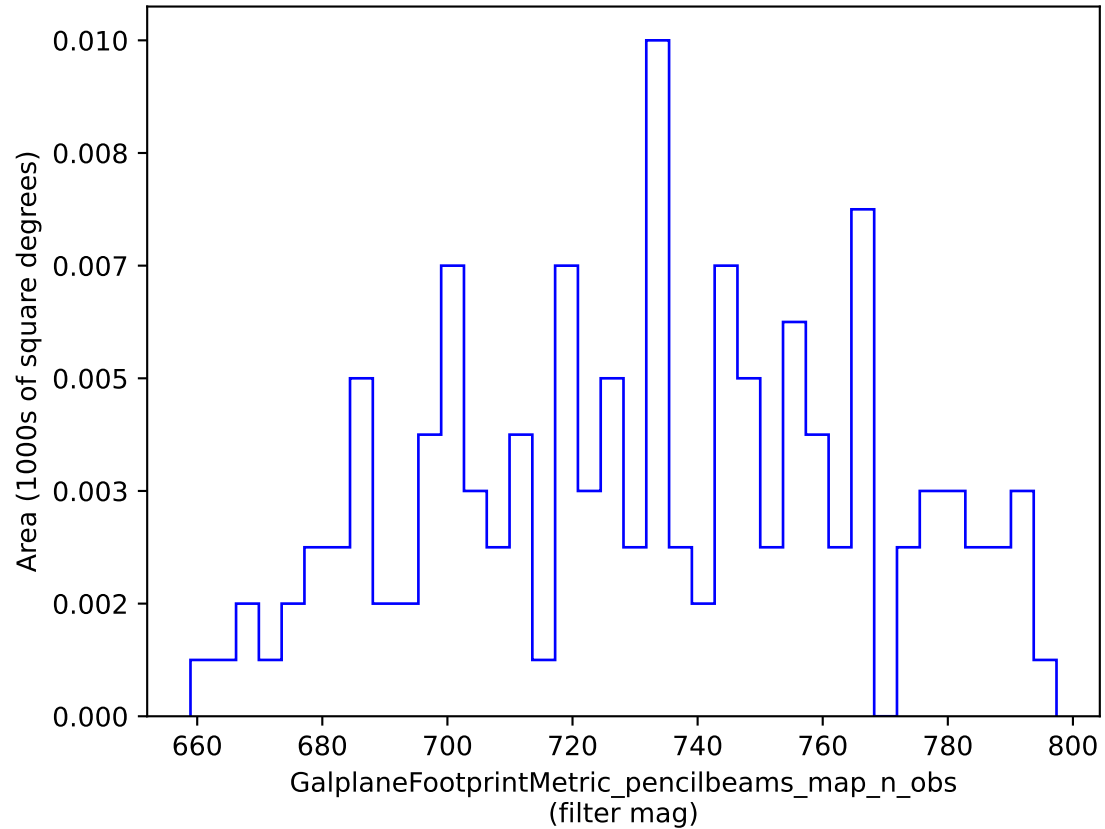
weather_cloudso8v3.4_10yrs : GalplaneFootprintMetric_pencilbeams_map_n_obs
