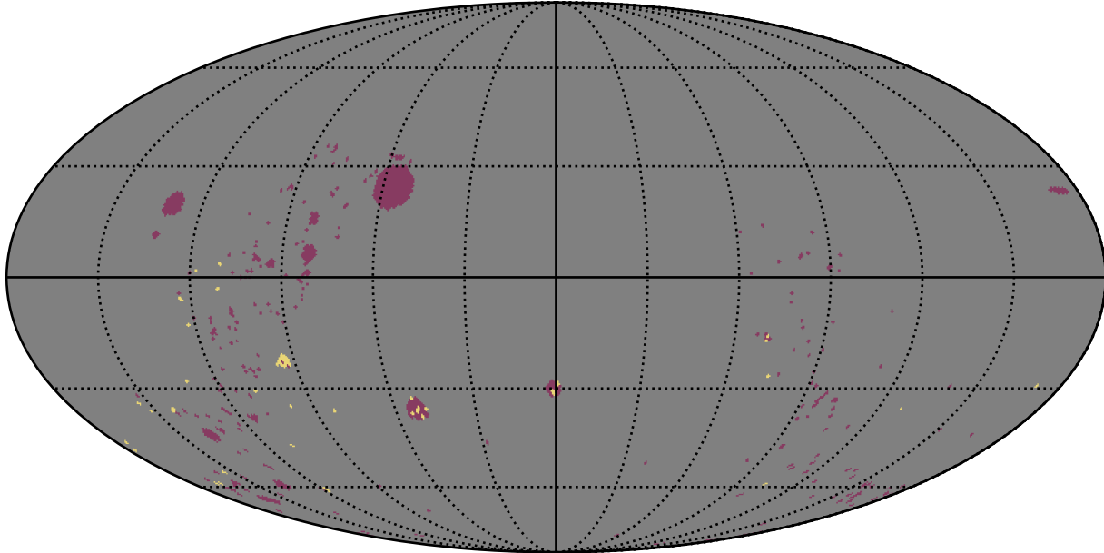
weather_cloudso8v3.4_10yrs : GalplaneFootprintMetric_open_clusters_map_Tau_5_0
