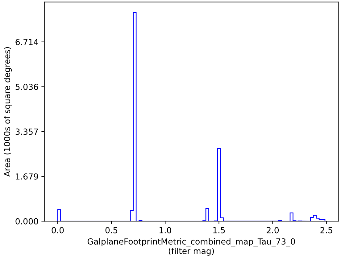
weather_cloudso8v3.4_10yrs : GalplaneFootprintMetric_combined_map_Tau_73_0
