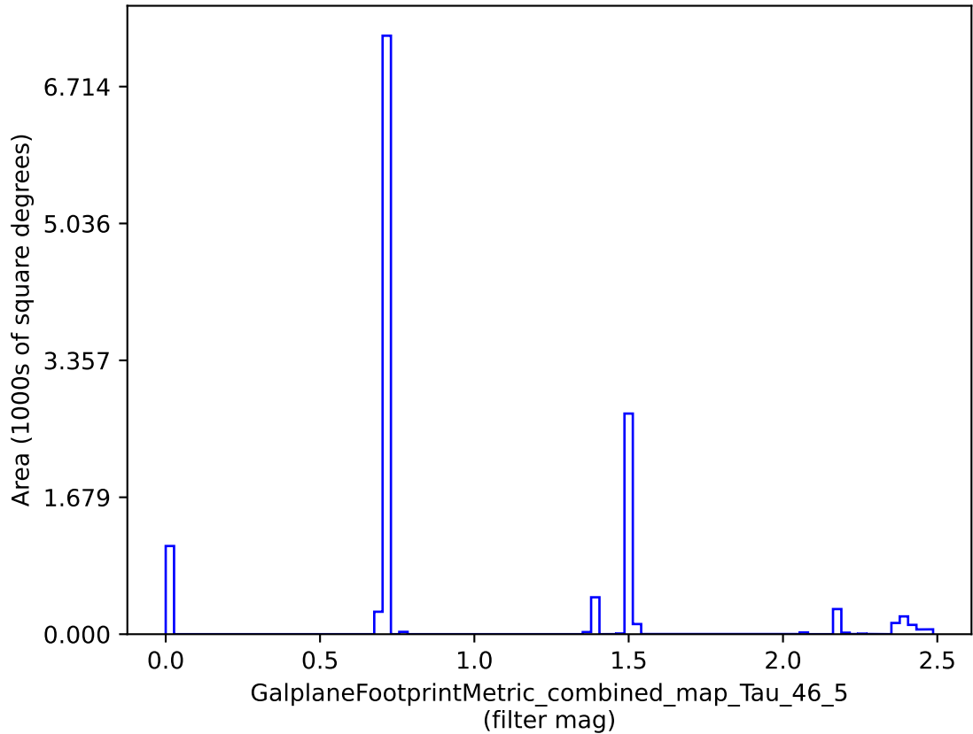
weather_cloudso8v3.4_10yrs : GalplaneFootprintMetric_combined_map_Tau_46_5
