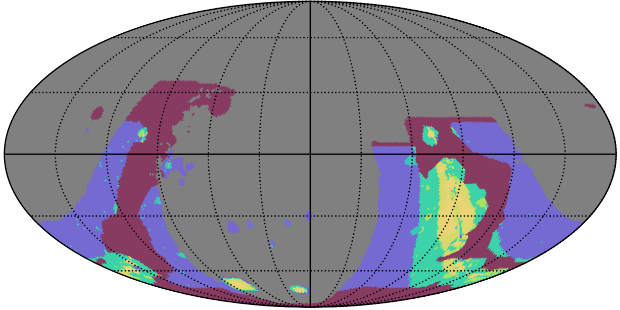
weather_cloudso8v3.4_10yrs : GalplaneFootprintMetric_combined_map_Tau_11_0
