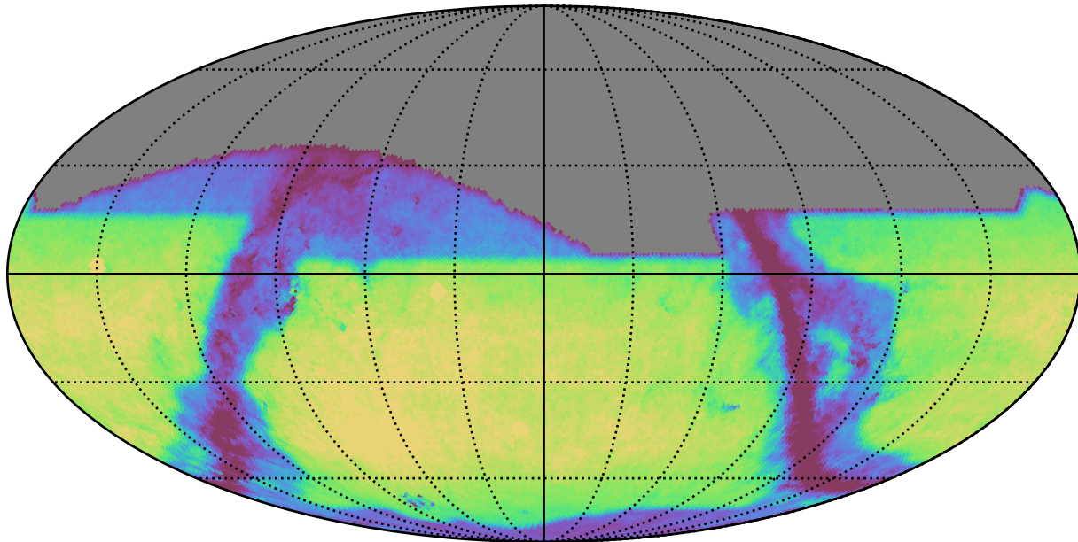
weather_cloudso8v3.4_10yrs z: GalaxyCountsMetricExtended
