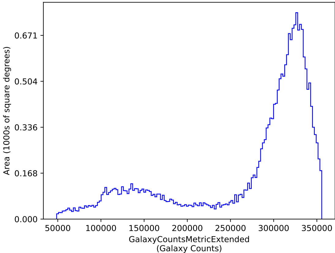
weather_cloudso8v3.4_10yrs y: GalaxyCountsMetricExtended
