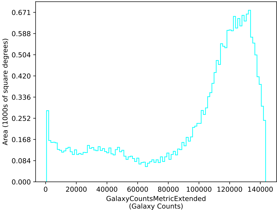
weather_cloudso8v3.4_10yrs u: GalaxyCountsMetricExtended
