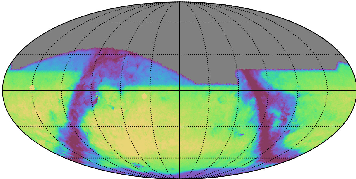
weather_cloudso8v3.4_10yrs r: GalaxyCountsMetricExtended
