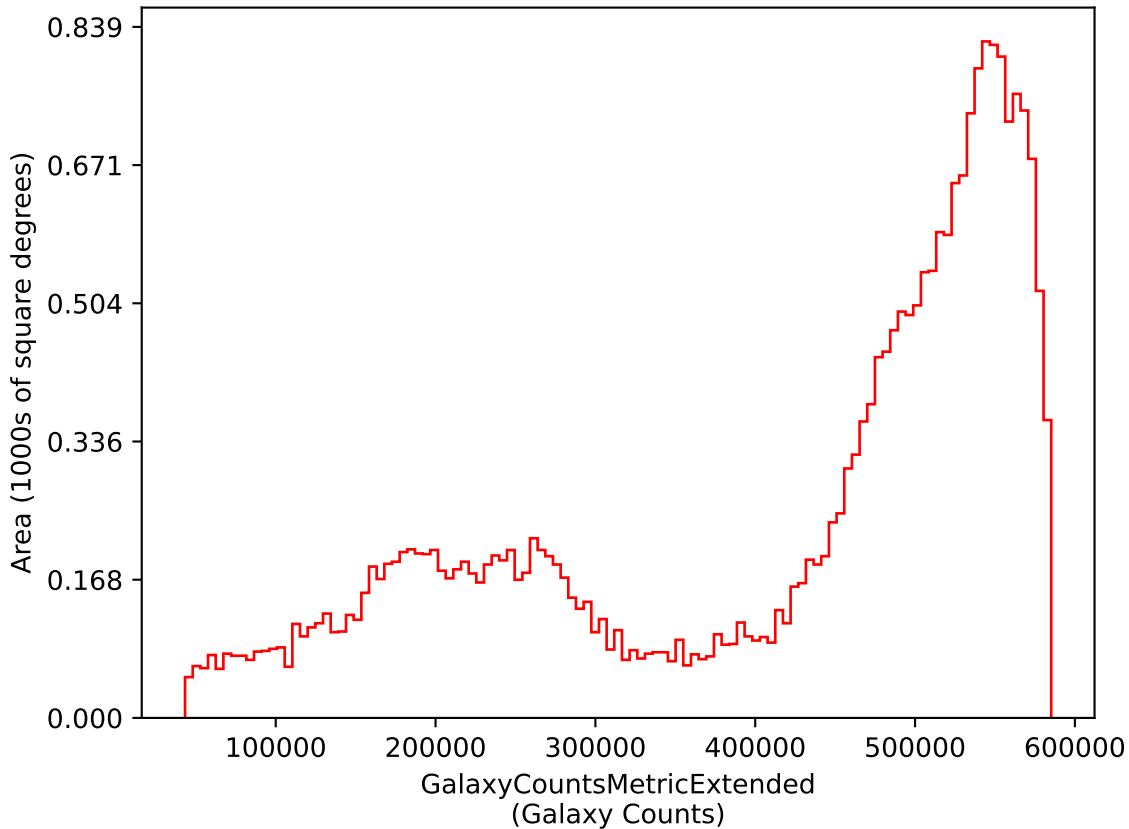
weather_cloudso8v3.4_10yrs i: GalaxyCountsMetricExtended
