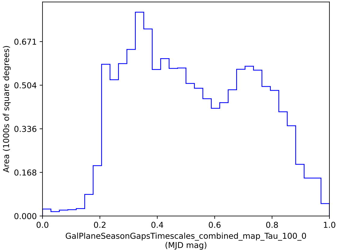
weather_cloudso8v3.4_10yrs : GalPlaneSeasonGapsTimescales_combined_map_Tau_100_0
