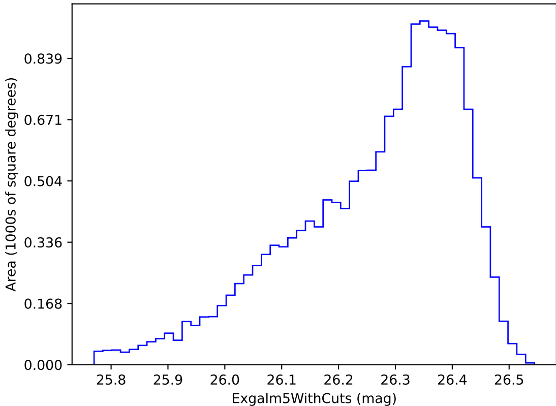
weather_cloudso8v3.4_10yrs i band non-DD year 8: Exgalml5WithCuts
