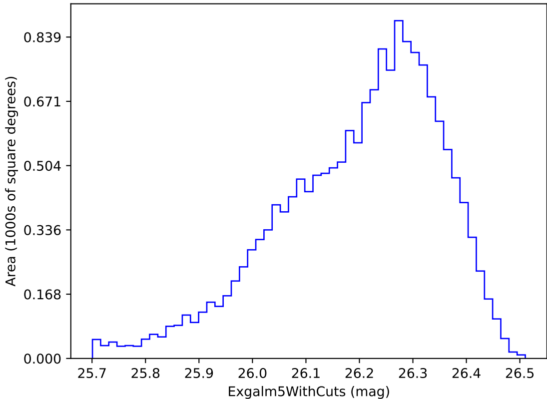
weather_cloudso8v3.4_10yrs i band non-DD year 7: Exgalml5WithCuts
