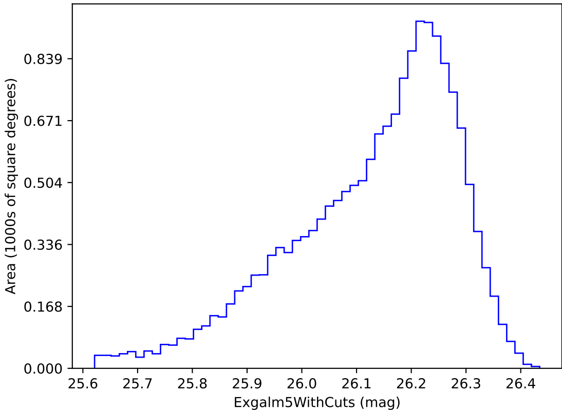
weather_cloudso8v3.4_10yrs i band non-DD year 6: ExgalM5WithCuts
