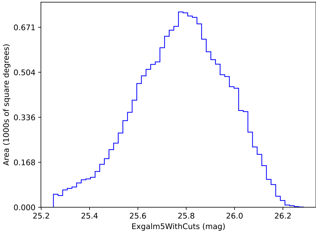
weather_cloudso8v3.4_10yrs i band non-DD year 3: Exgal5WithCuts
