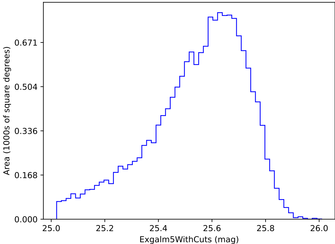
weather_cloudso8v3.4_10yrs i band non-DD year 2: Exgalml5WithCuts
