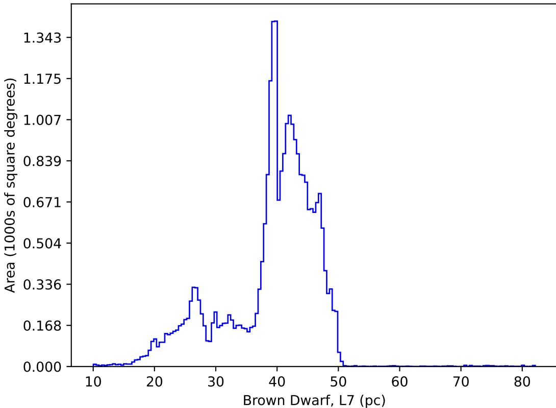
weather_cloudso8v3.4_10yrs : Brown Dwarf, L7
