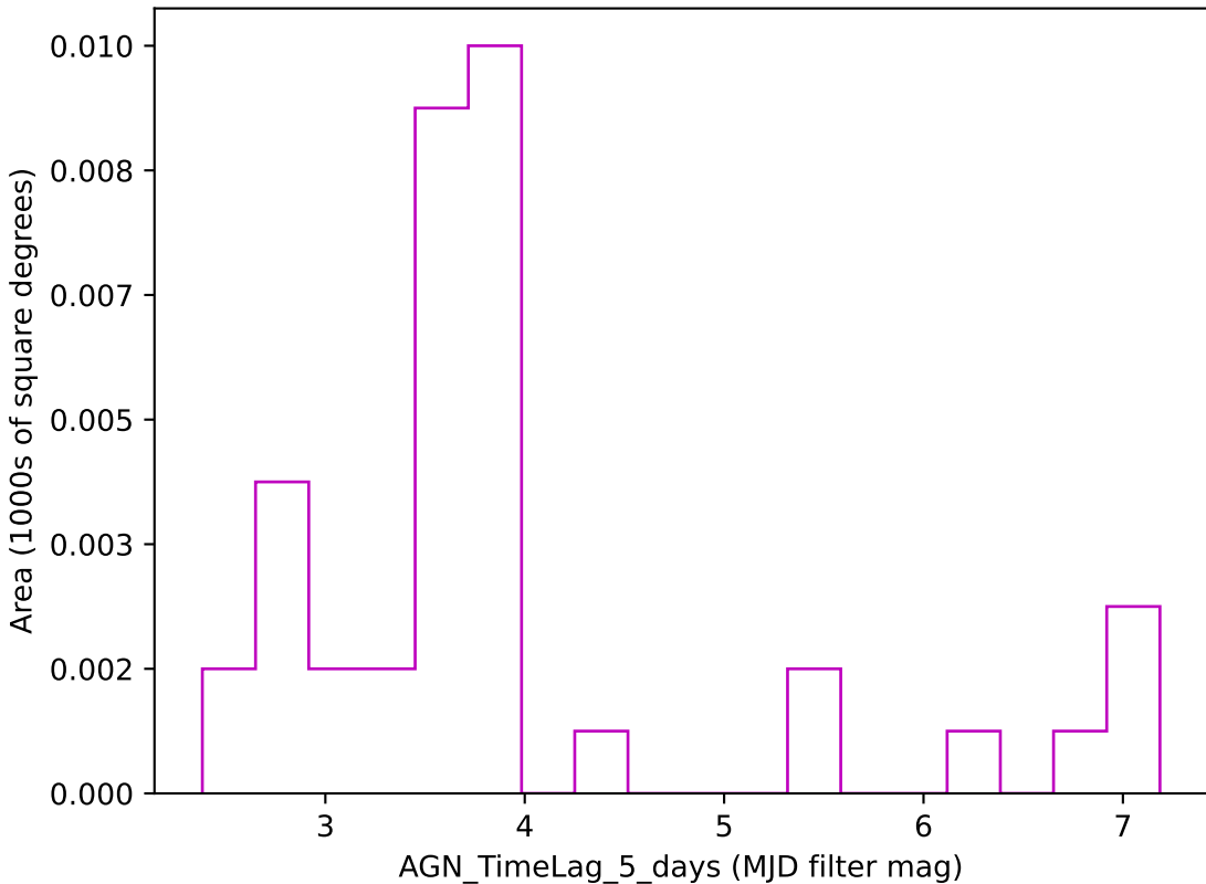
weather_cloudso8v3.4_10yrs z band: AGN_TimeLag_5_days
