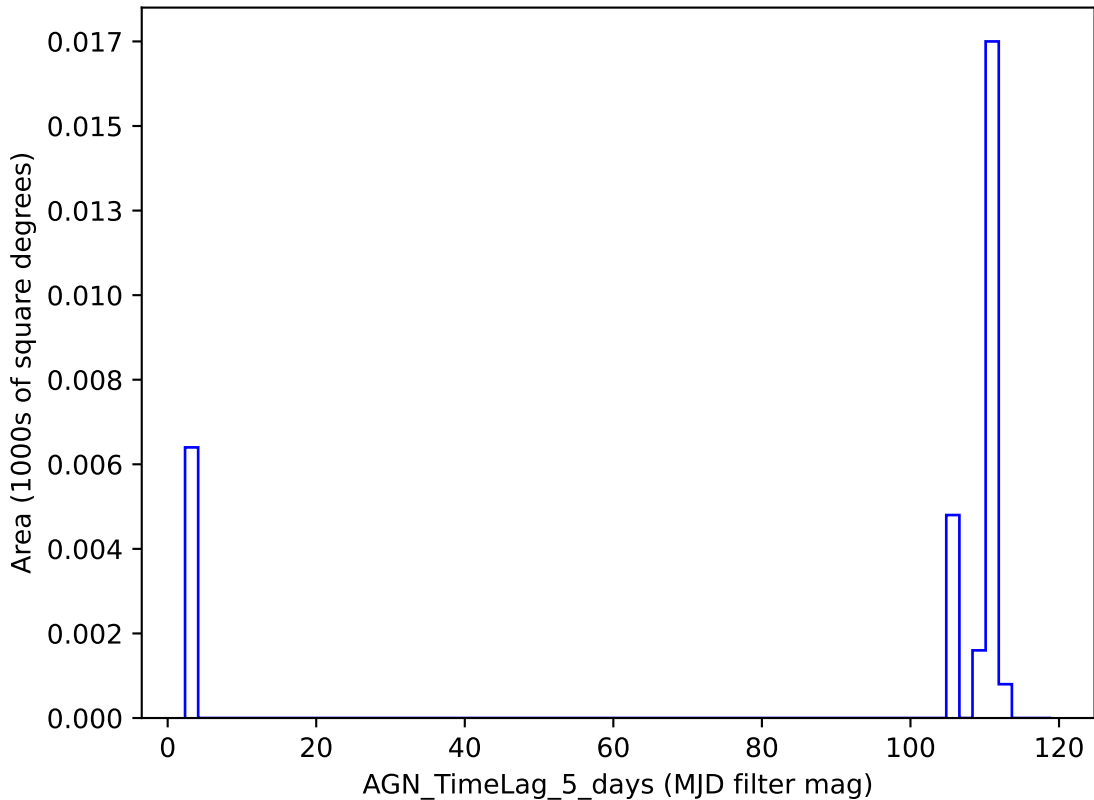
weather_cloudso8v3.4_10yrs y band: AGN_TimeLag_5_days
