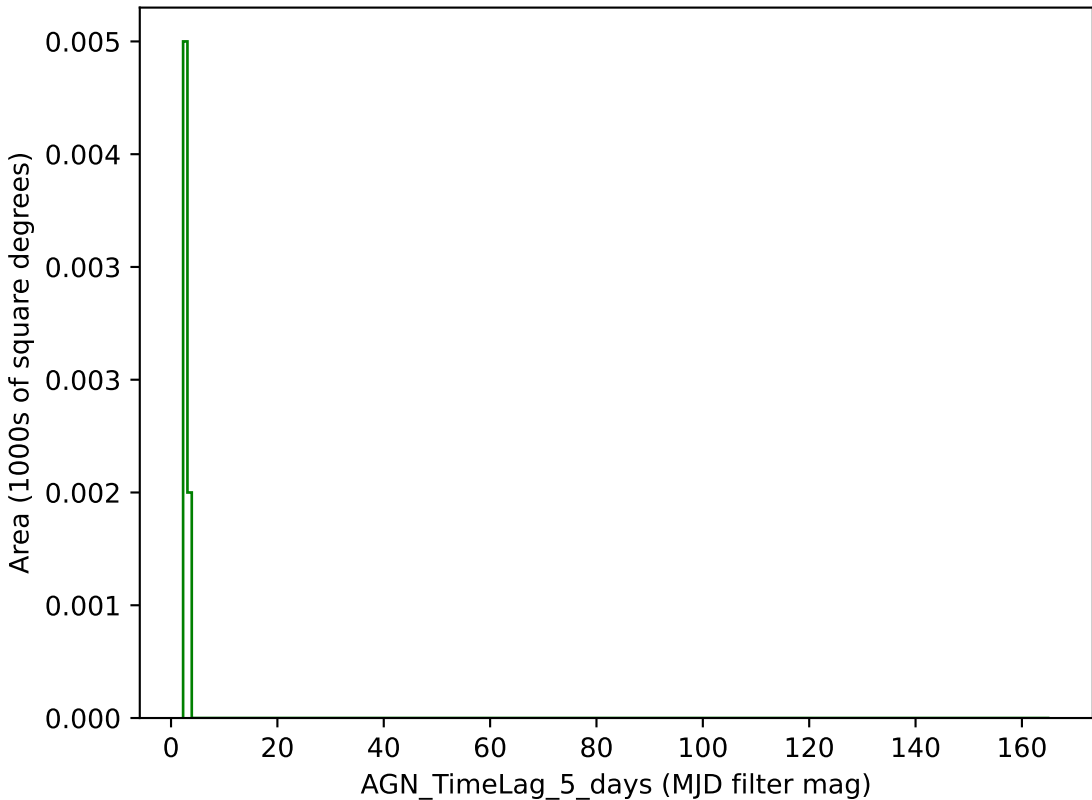
weather_cloudso8v3.4_10yrs g band: AGN_TimeLag_5_days
