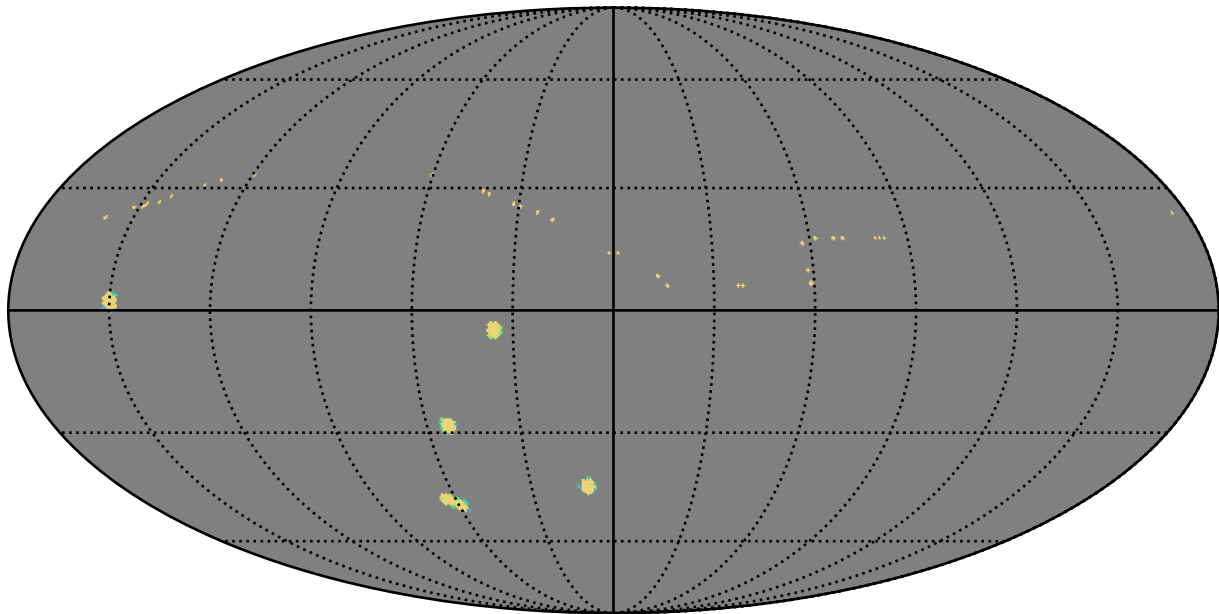
weather_cloudso8v3.4_10yrs all bands: AGN_TimeLag_5_days
