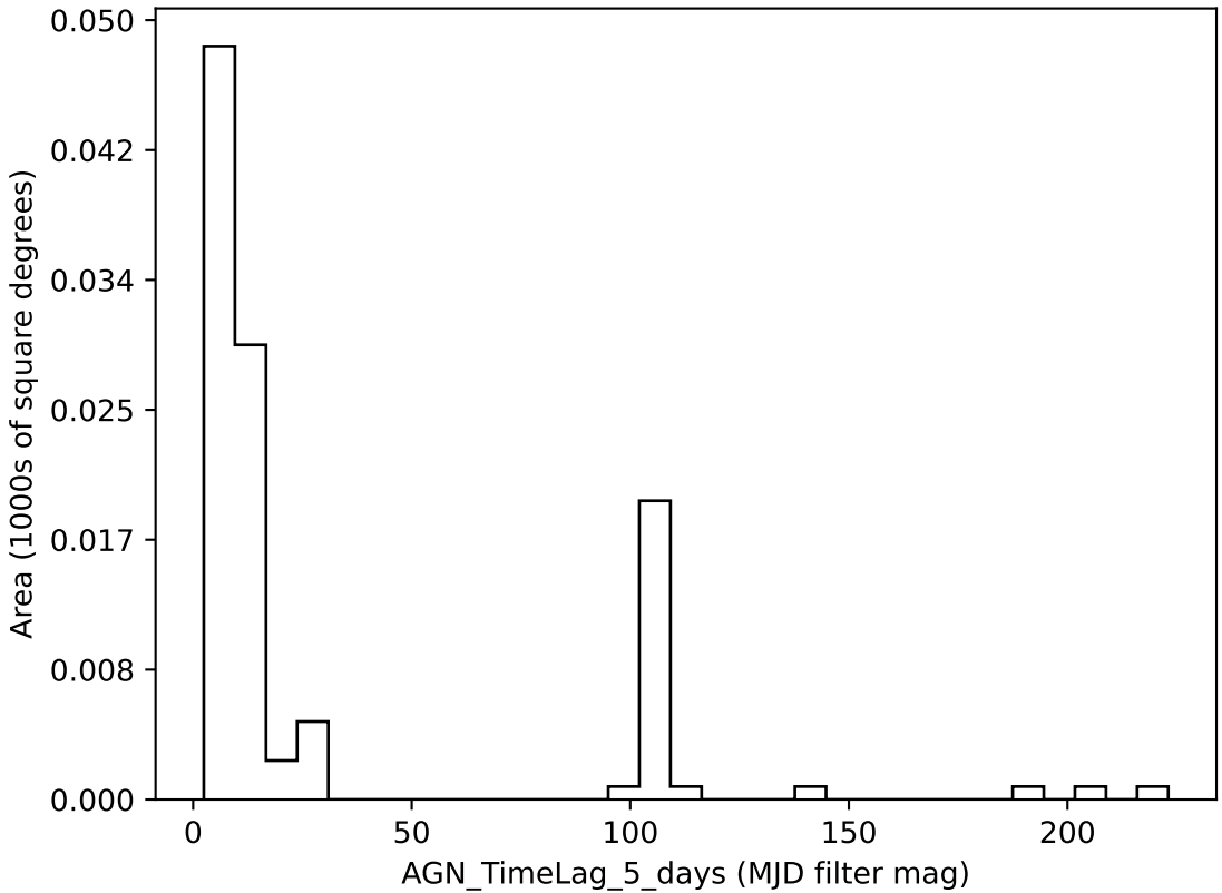
weather_cloudso8v3.4_10yrs all bands: AGN_TimeLag_5_days
