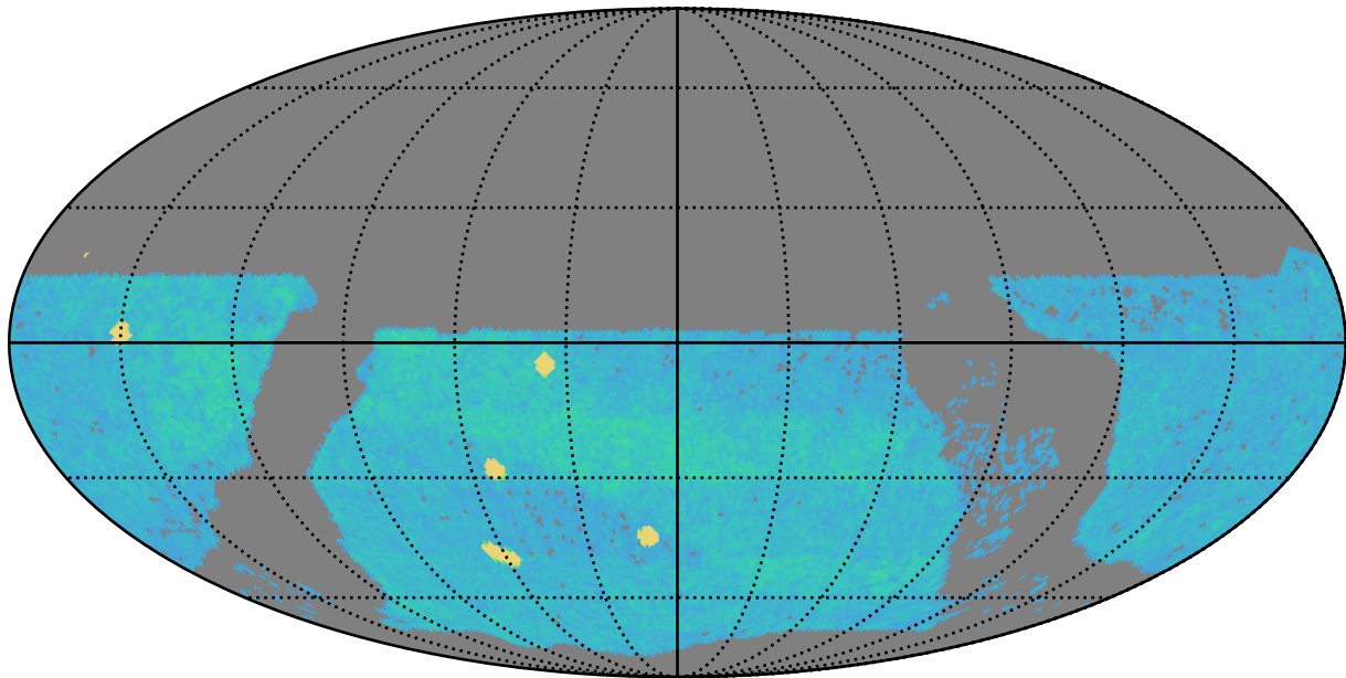
weather_cloudso8v3.4_10yrs z band: AGN_TimeLag_100_days
