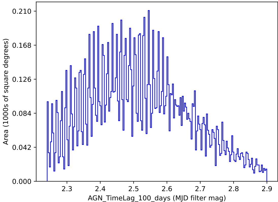
weather_cloudso8v3.4_10yrs y band: AGN_TimeLag_100_days
