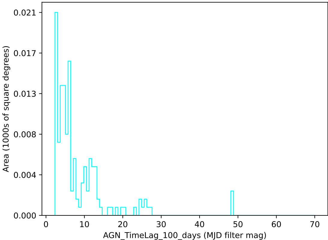
weather_cloudso8v3.4_10yrs u band: AGN_TimeLag_100_days
