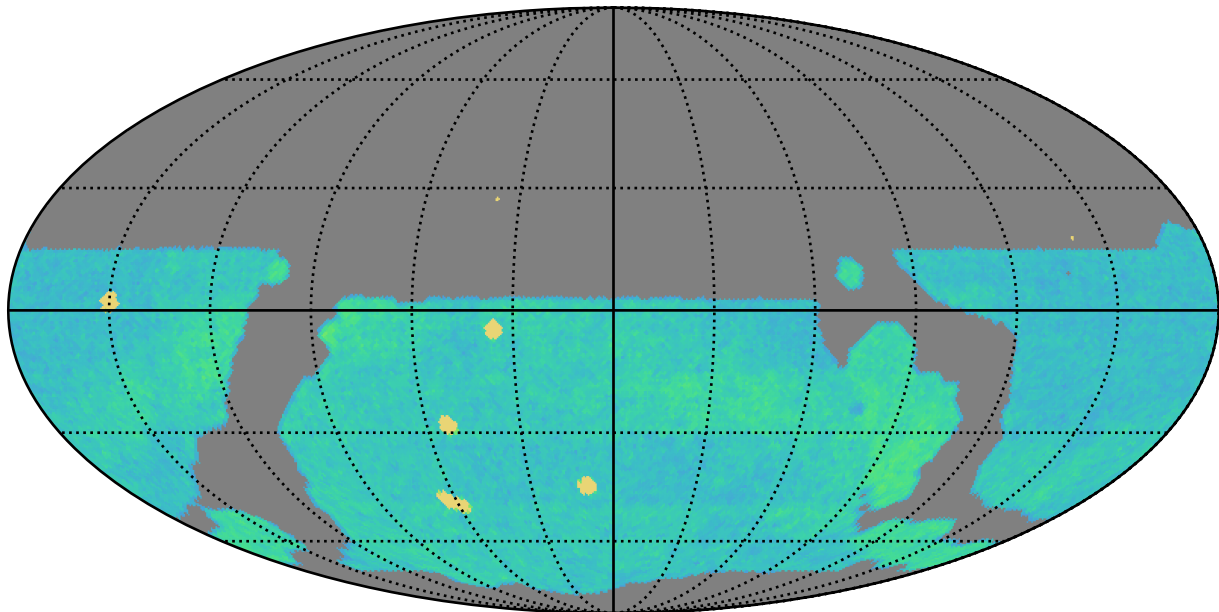
weather_cloudso8v3.4_10yrs r band: AGN_TimeLag_100_days
