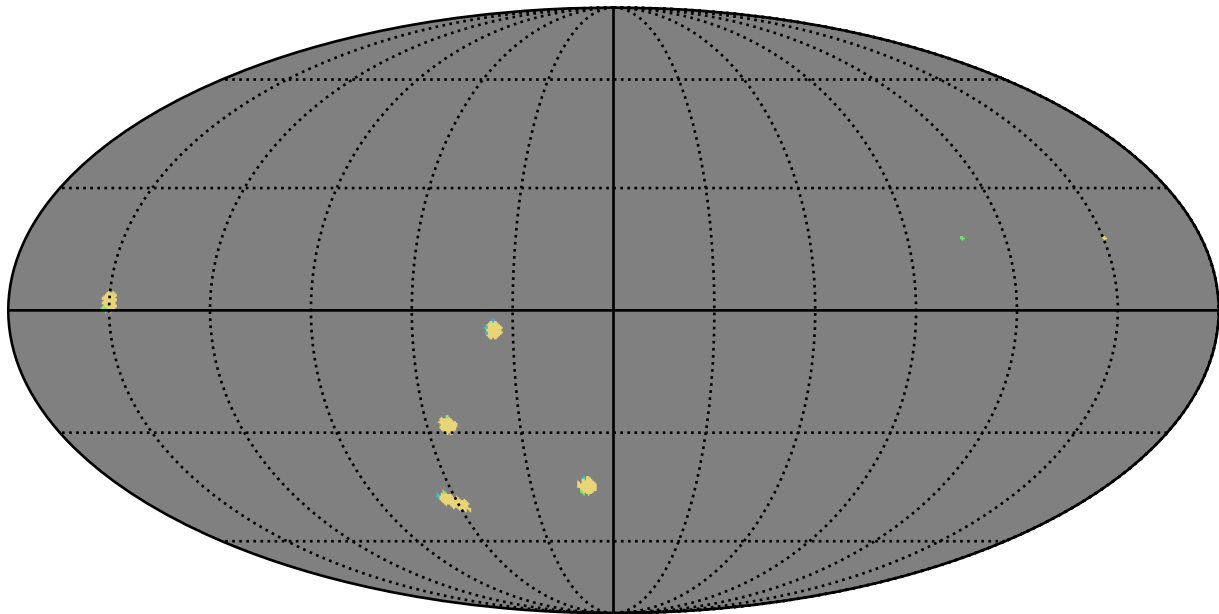
weather_cloudso8v3.4_10yrs g band: AGN_TimeLag_100_days
