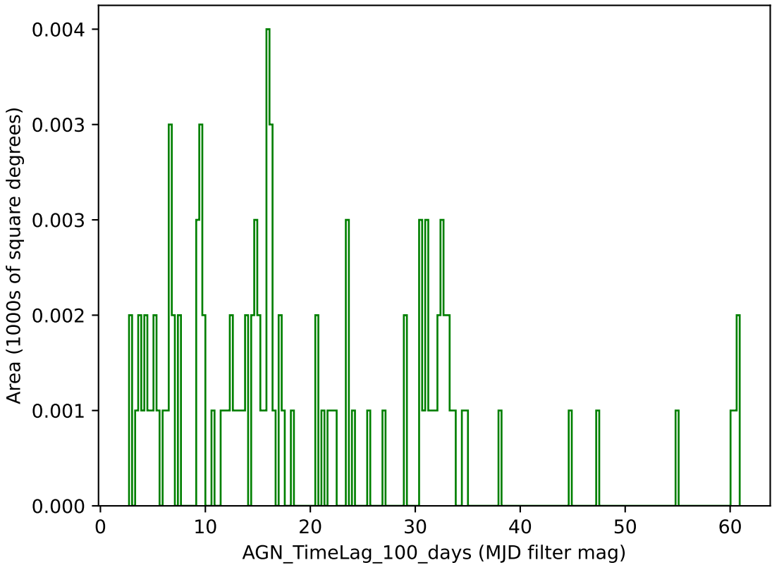
weather_cloudso8v3.4_10yrs g band: AGN_TimeLag_100_days
