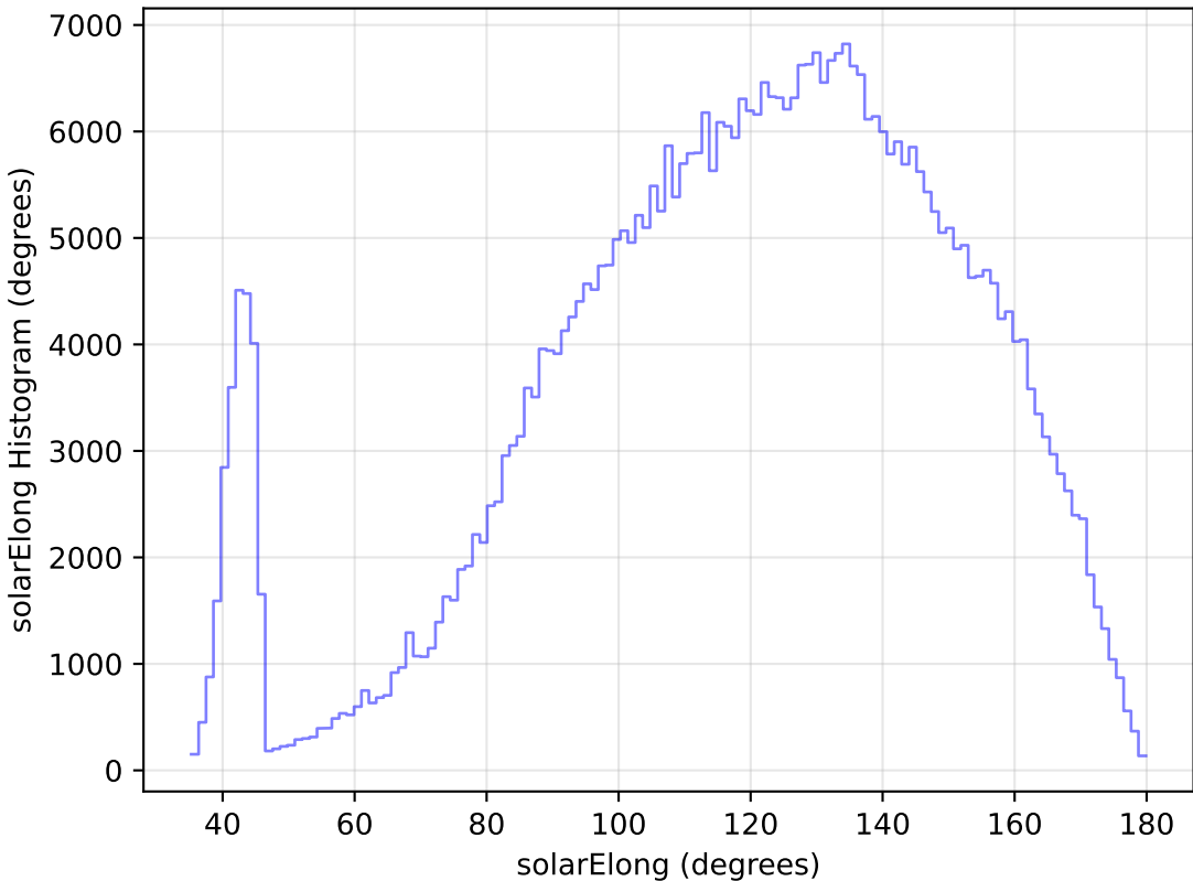
weather_cloudso8v3.4_10yrs WFD z band: solarElong Histogram
