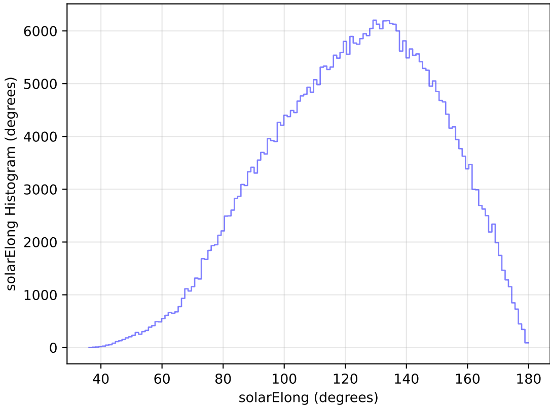
weather_cloudso8v3.4_10yrs WFD y band: solarElong Histogram
