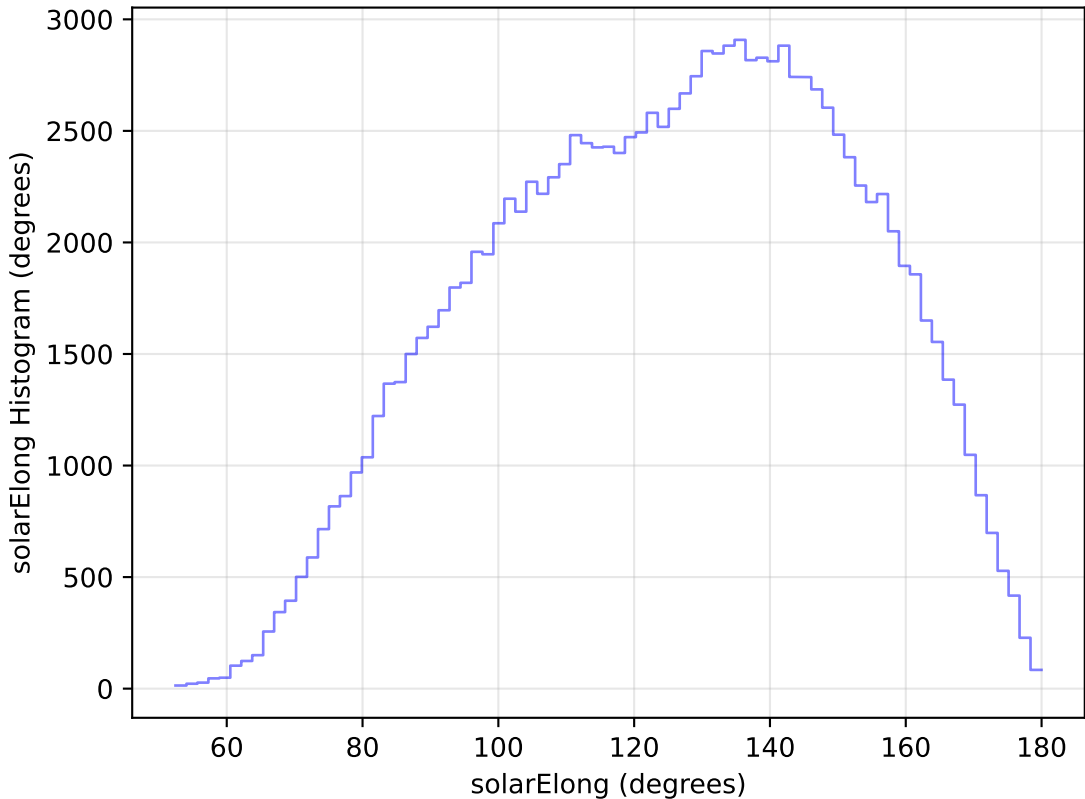
weather_cloudso8v3.4_10yrs WFD u band: solarElong Histogram
