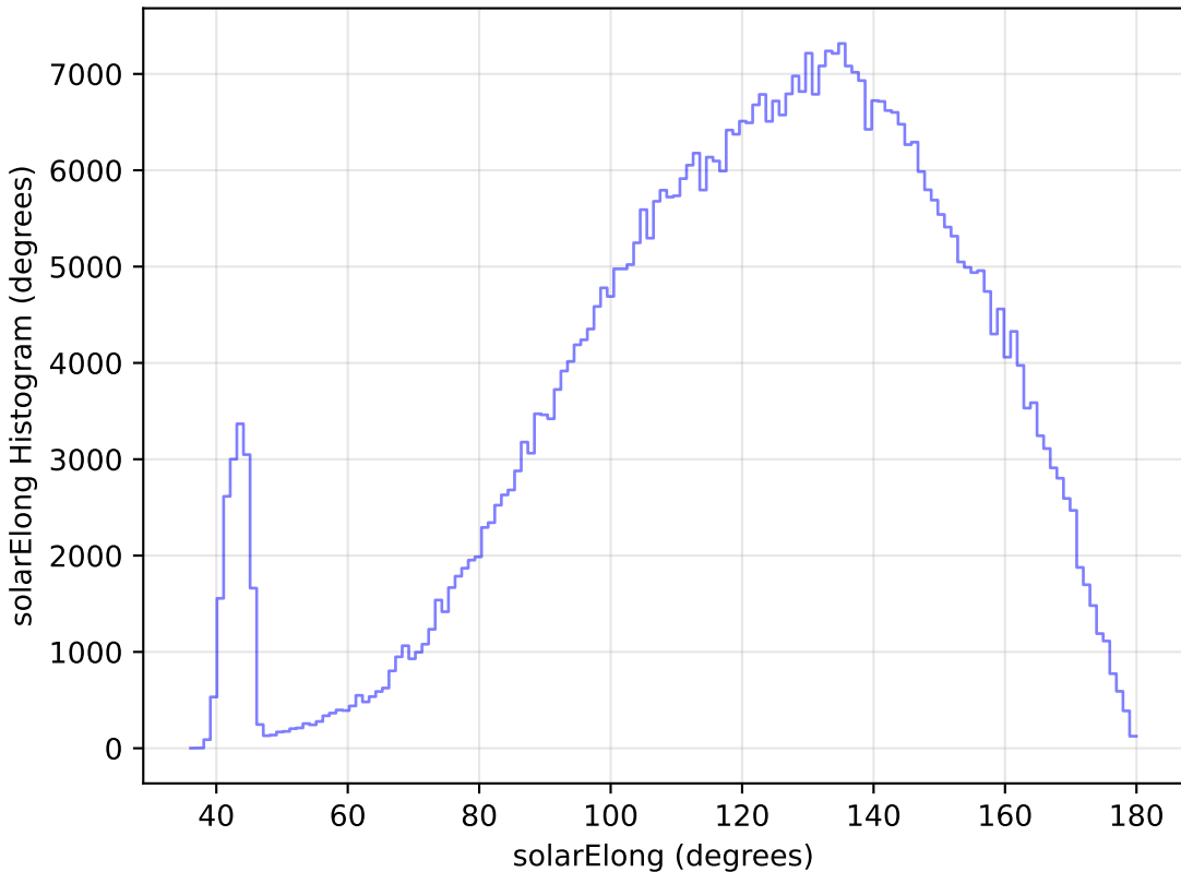
weather_cloudso8v3.4_10yrs WFD r band: solarElong Histogram
