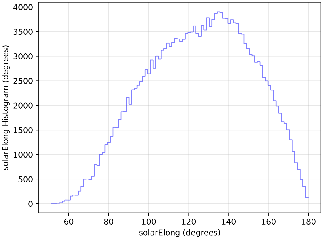
weather_cloudso8v3.4_10yrs WFD g band: solarElong Histogram
