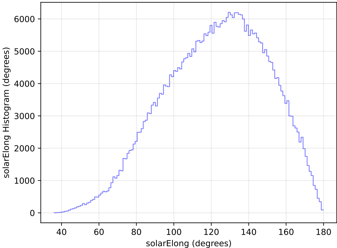
weather_cloudso8v3.4_10yrs All sky y band: solarElong Histogram
