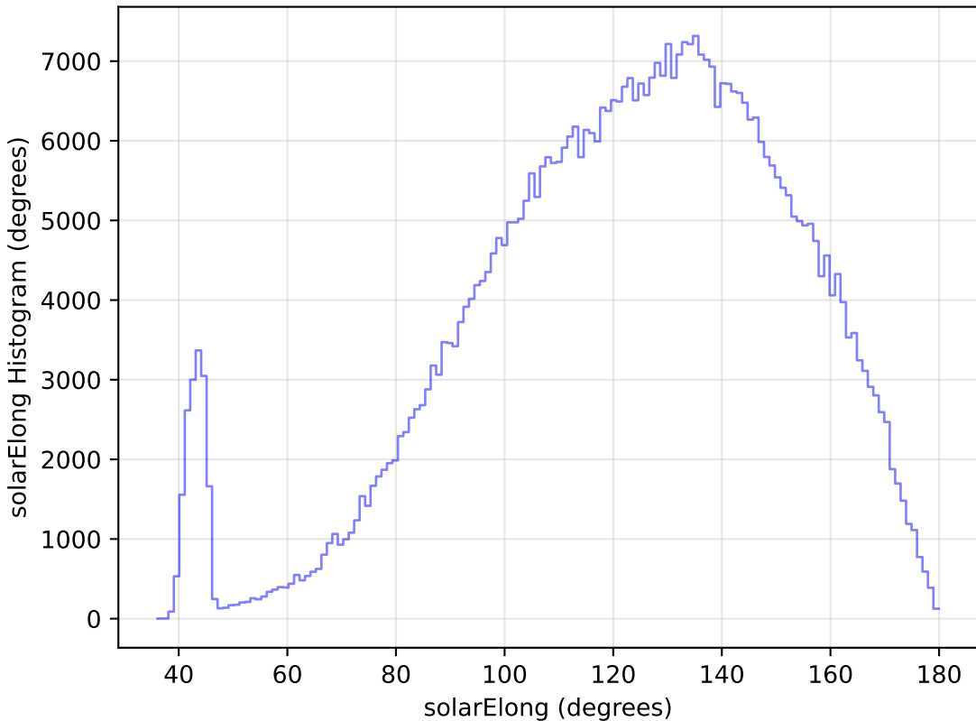
weather_cloudso8v3.4_10yrs All sky r band: solarElong Histogram
