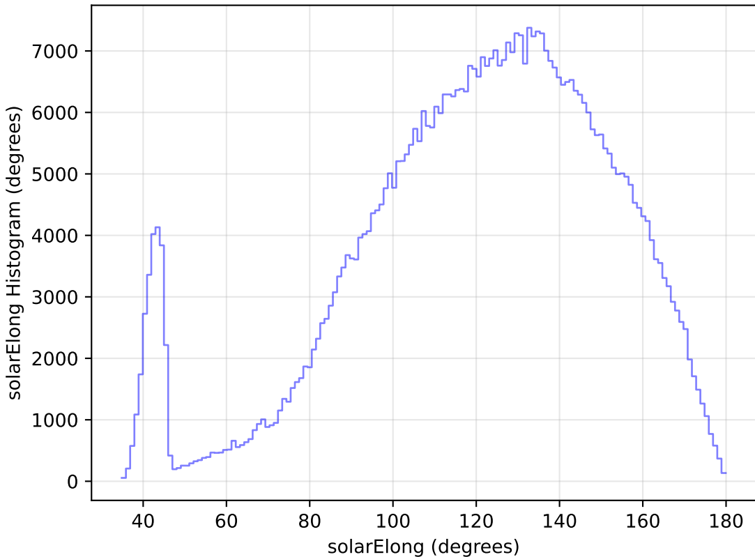
weather_cloudso8v3.4_10yrs All sky i band: solarElong Histogram
