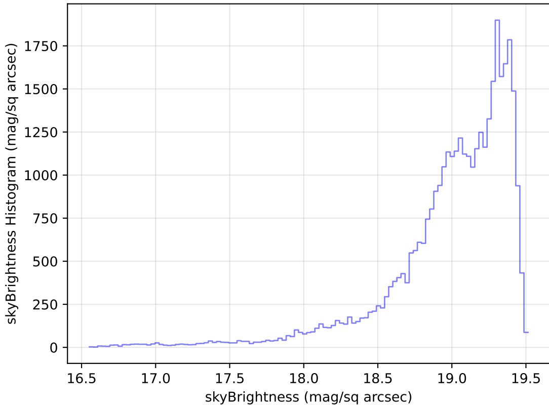
weather_cloudso8v3.4_10yrs Yr 1 z band: skyBrightness Histogram
