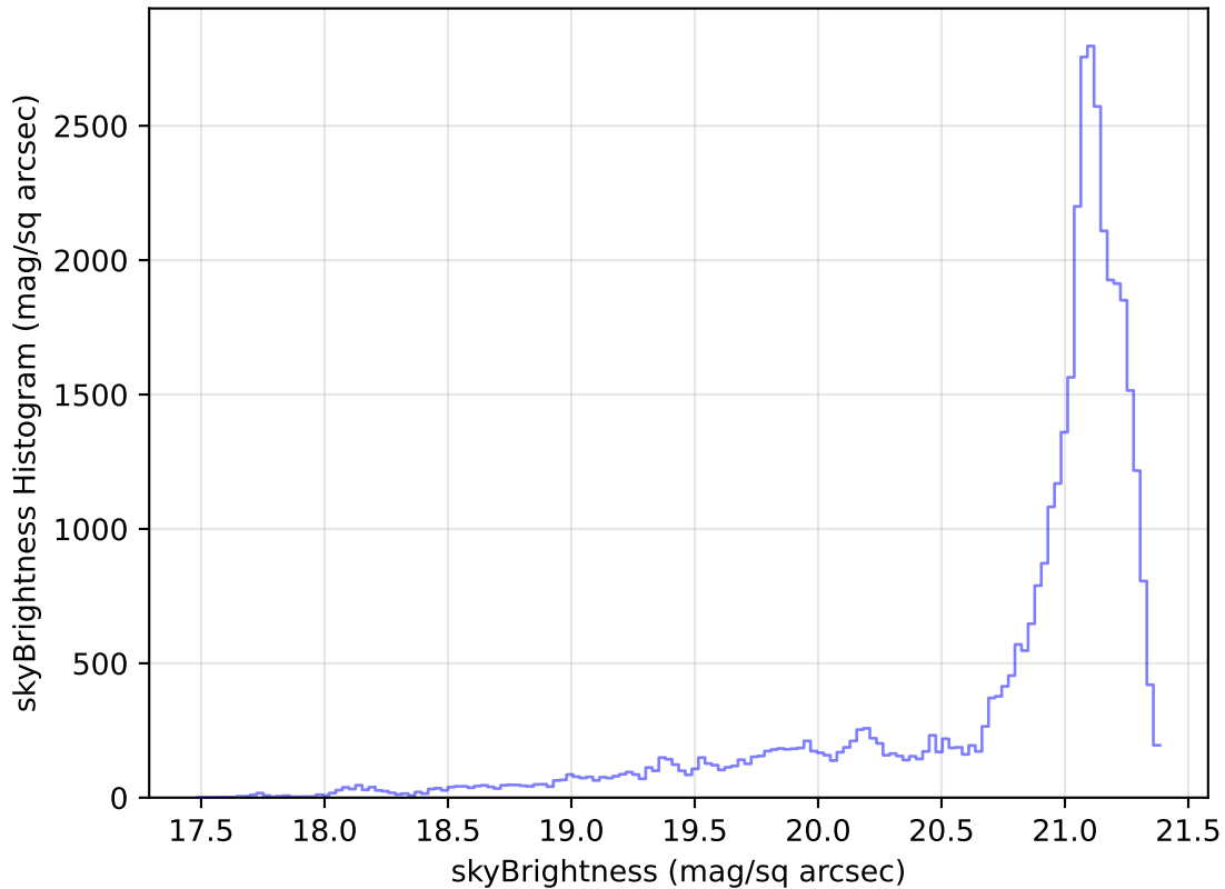
weather_cloudso8v3.4_10yrs Yr 1 r band: skyBrightness Histogram
