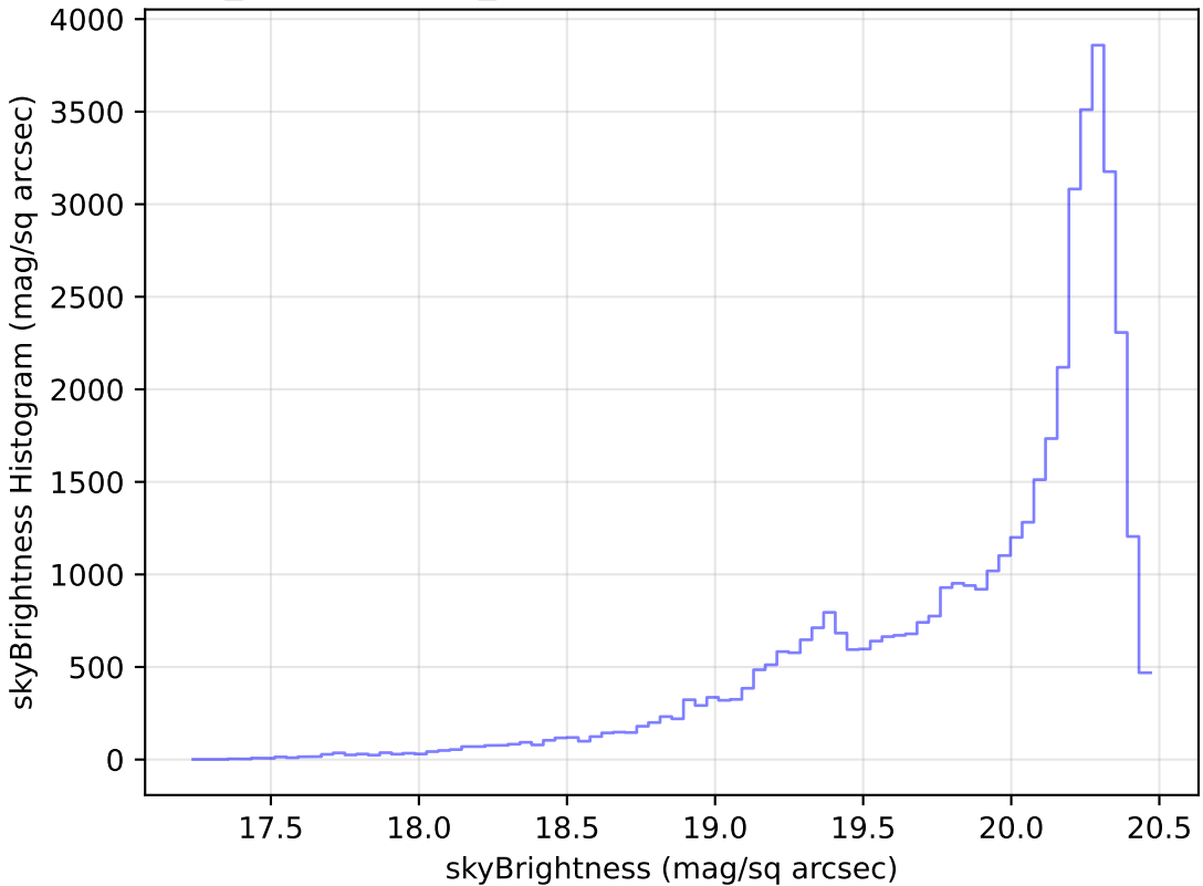
weather_cloudso8v3.4_10yrs Yr 1 i band: skyBrightness Histogram
