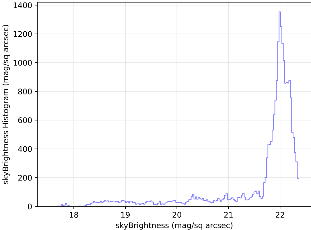
weather_cloudso8v3.4_10yrs Yr 1 g band: skyBrightness Histogram
