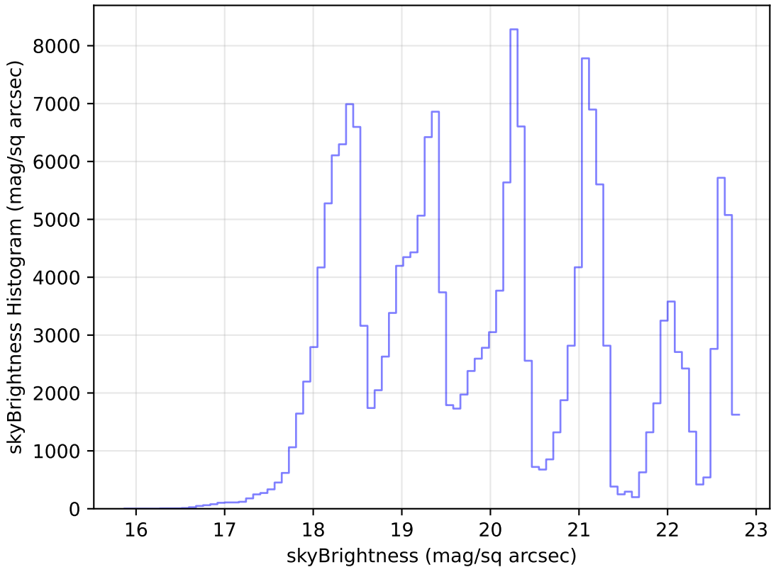
weather_cloudso8v3.4_10yrs Yr 1 all bands: skyBrightness Histogram
