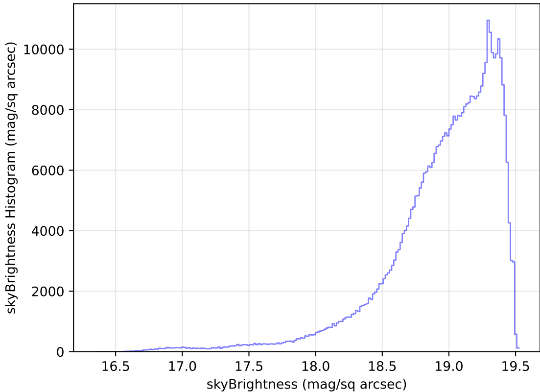
weather_cloudso8v3.4_10yrs WFD z band: skyBrightness Histogram
