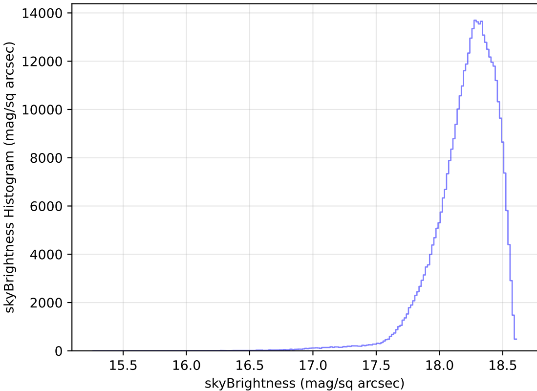
weather_cloudso8v3.4_10yrs WFD y band: skyBrightness Histogram
