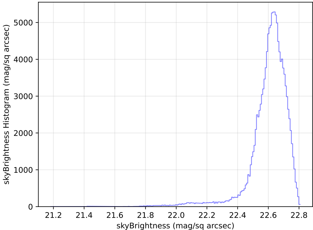
weather_cloudso8v3.4_10yrs WFD u band: skyBrightness Histogram
