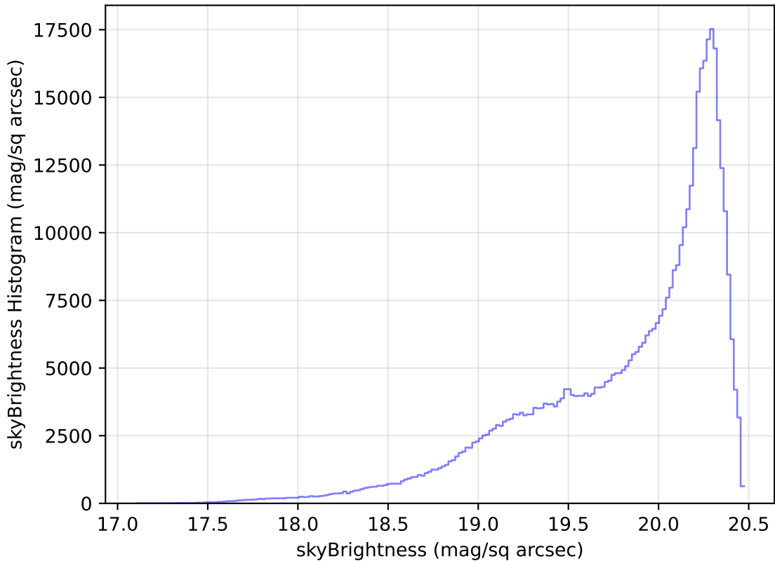
weather_cloudso8v3.4_10yrs WFD i band: skyBrightness Histogram
